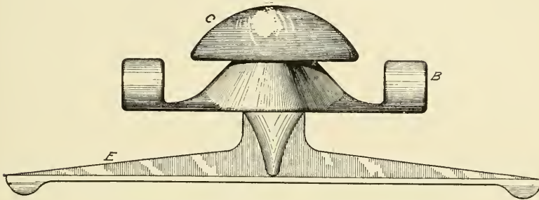
Fig. 181. Hanger and Ear for Round Trolley Wire
